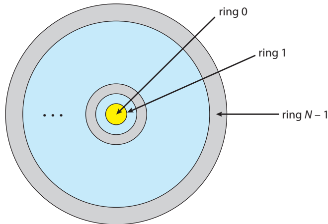
Figure 17.1 Protection-ring structure.
