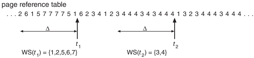
Figure 10.22 Working-set model.
