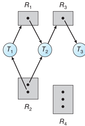
Figure 8.4 Resource-allocation graph.
