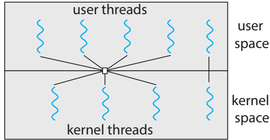
Figure 4.10 Two-level model.
