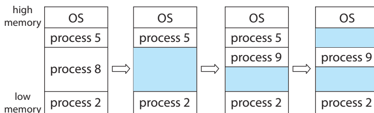
Figure 9.7 Variable partition.
