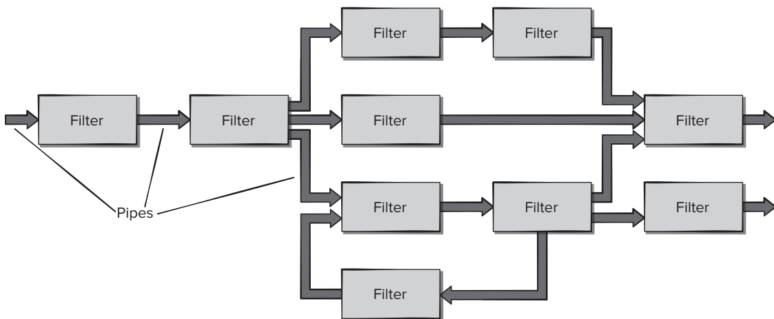
FIGURE 10.2 Data-flow architecture
